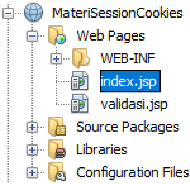
Gambar 204. File Validasi.jsp
