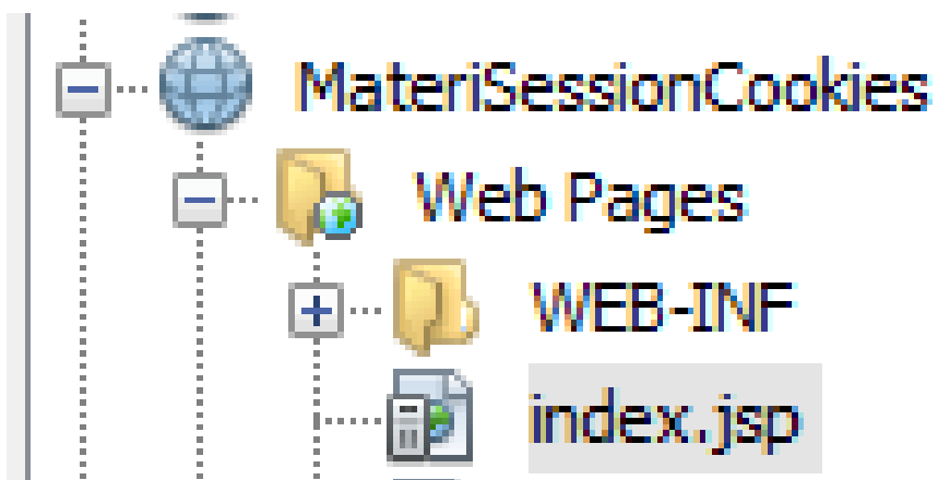
Gambar 200. File Index.jsp
