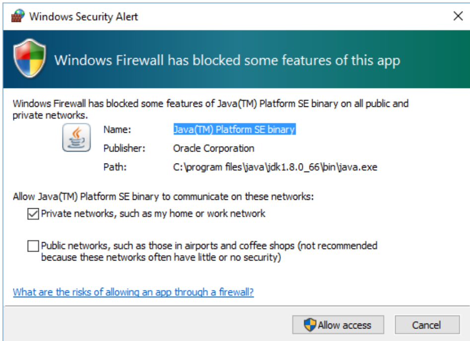
Gambar 207. Security Alert
