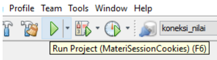
Gambar 206. Proses Run
